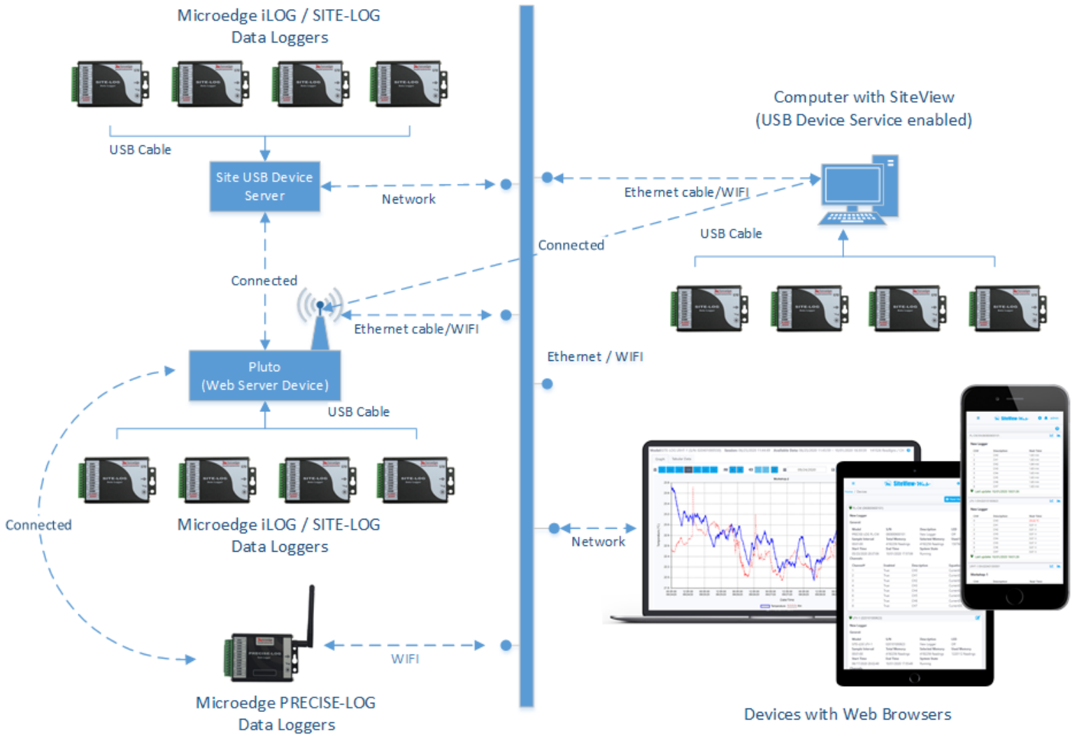
Data Logger Network Option – Pluto as Web Server
