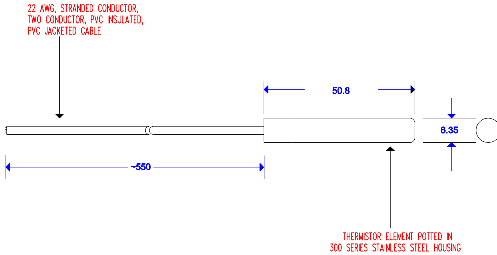
Fig. 1.4: A927ZET External probe
