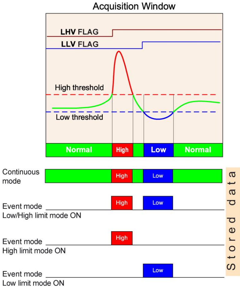
Fig. 2.1: A927ZET Sampling Operating Modes
