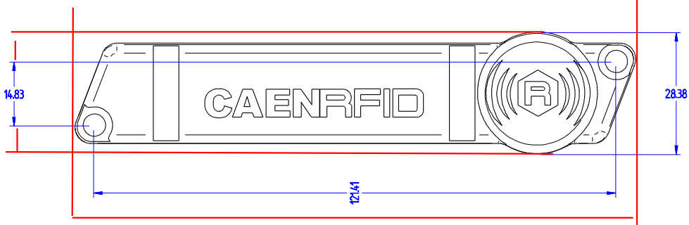
Fig. 1.3: A927ZET Technical drawings
